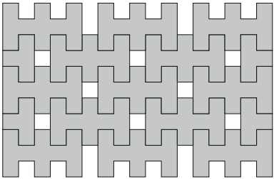
LAYING SCHEME 1 43,20 pcs / sqm
